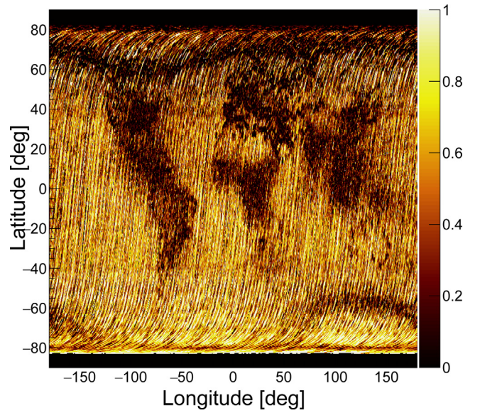
Fig. 4. Ratio of active time over the total amount of transit time as a function of geographical location.
