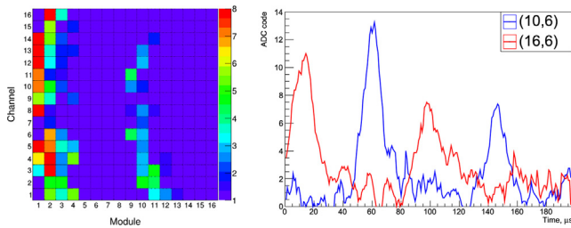
Fig. 10. A double ELVE measured by the TUS detector on 10th April, 2017. Left: pixel map, two bright rings are seen. Right: the waveforms of the two channels (10,6) and (16,6) (blue and red lines), each comprise two peaks with a time delay of \sim 85 \mu s.
