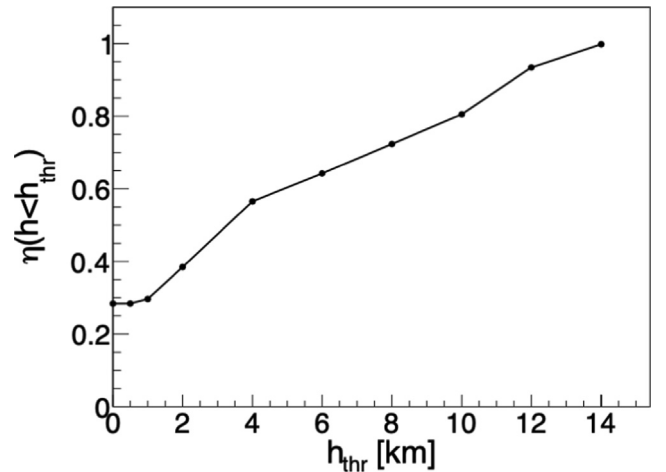
Fig. 5. Fraction of triggers with cloud top height below h_{thr} (see the text for details).
