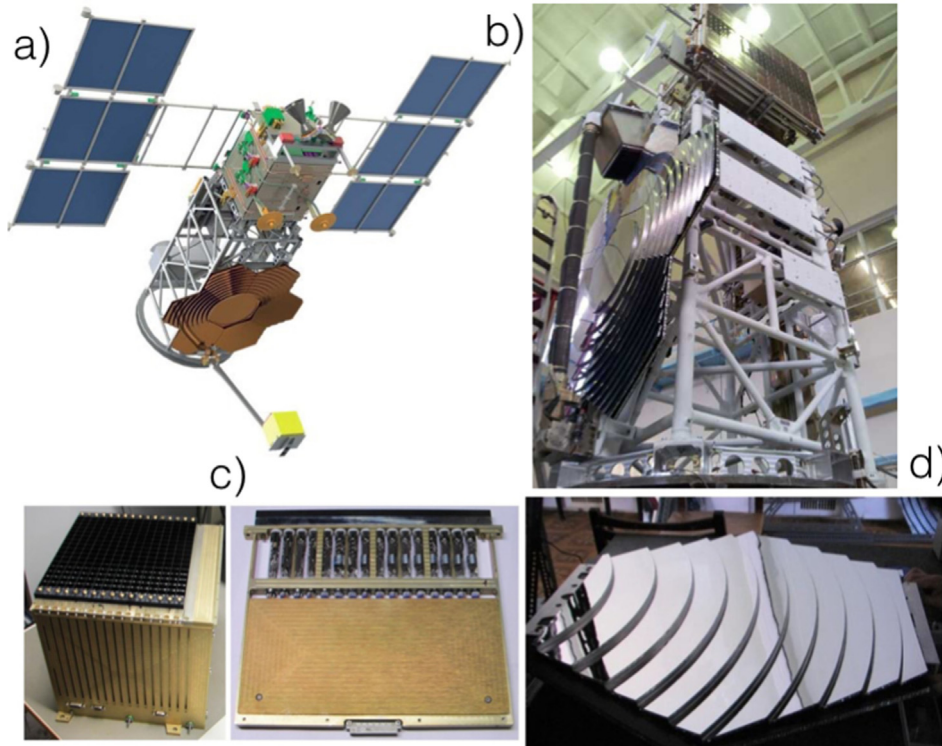
Fig. 1. (a) Artist's view of the TUS detector on board the Lomonosov satellite; (b) TUS on board the Lomonosov satellite during preflight preparations at cosmodrome Vostochny; (c) TUS focal surface; (d) a segment of the TUS Fresnel mirror.
