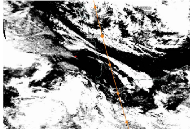
Fig. 14. Cloud cover from the MODIS Terra satellite at 1509 UTC, white parts indicate cloud cover, black parts indicate clear sky, while the orange line is the orbit track with times of acquisition. The red dot indicates the position of TUS170426 event.
