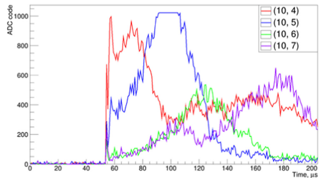
Fig. 11. Waveforms of the four active channels indicated in the inset for the TUS160905 event.
