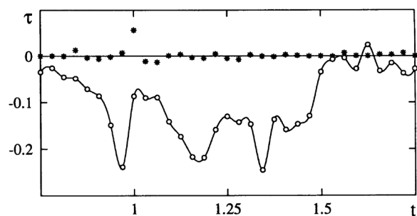
Fig. 10. Specific torques acting on the gas at the center of the face-on disk in a gas-rich equal-mass merger between two disk galaxies, as a function of time (with the units of length, mass, and time being roughly 40 kpc, 2.2 \times 10^{11} M_{\odot} , and 250 Myr, respectively). In this relatively low-resolution simulation, the gravitational torques exerted on the gas by the rest of the system (open circles) are much stronger than those due to hydrodynamic forces (star symbols), as opposed to the high-resolution case described in Figs. 7–9. From Barnes and Hernquist (1991).
