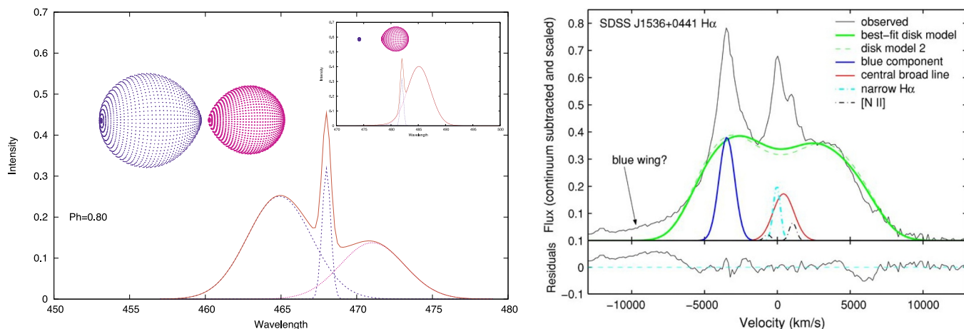
Fig. 16. Left panel: H\beta emission-line profile emitted from the SMBHB system when both black holes have the BLR, while in the inset the line profile when only one component has the BLR is shown. Adapted from Popović (2012). Right panel: H\alpha emission line (once the continuum spectrum is removed; solid black line) fitted by the disk model (solid green line). There are additionally two relatively broad peaks, reproduced using two Gaussian profiles (blue and red line), while the cyan dash-dotted line is the Gaussian fit to the narrow H\alpha component. The black dash-dotted lines are the Gaussian fits to [NII] \lambda 6548, 6583 lines, with fixed FWHM given by fitting [OIII] \lambda 4959, 5007. The dashed green line shows the disk model line with outer radius 8000 r_g , and the same inner radius and inclination as the best-fit solid green line. The black solid line in the lower panel shows the residuals. From Tang and Grindlay (2009).
