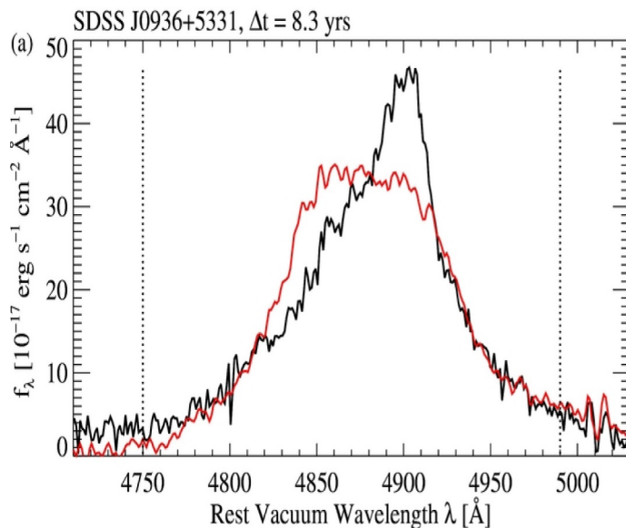
Fig. 18. SMBHB candidates identified through optical H \beta offset. Left panel: these candidates were selected on the basis of the presence of broad H \beta emission lines that are velocity shifted relative to the narrow [O III] \lambda\lambda 4959, 5007 emission lines. The dashed line marks the rest wavelength of H \beta , and the dotted lines mark \pm 5,000 and 10,000 \text{ km s}^{-1} relative to the dashed line. Thus, the broad H \beta peaks are offset by a few \times 1000 \text{ km s}^{-1} . This may be the observational consequence of a scenario where one of the BHs in a SMBHB is active and its orbital motion induces a periodic radial velocity shift in the broad H \beta emission line relative to the narrow lines in the spectrum. Such a system would likely have a sub-pc separation corresponding to a period of the order of decades to hundreds years. Adapted from Eracleous et al. (2012). Right Panel: example of the cross-correlation analysis applied to measure the velocity shift of the broad H \beta between two epochs. The broad H \beta in the SDSS spectrum is shown in black, while the follow-up observation is in red. The spectral range of the cross-correlation analysis is marked by the dotted vertical lines. Negative values of the cross-correlation analysis mean that the emission line in the follow-up spectrum needs to be blue-shifted to match the SDSS spectrum. From Liu et al. (2014b).
