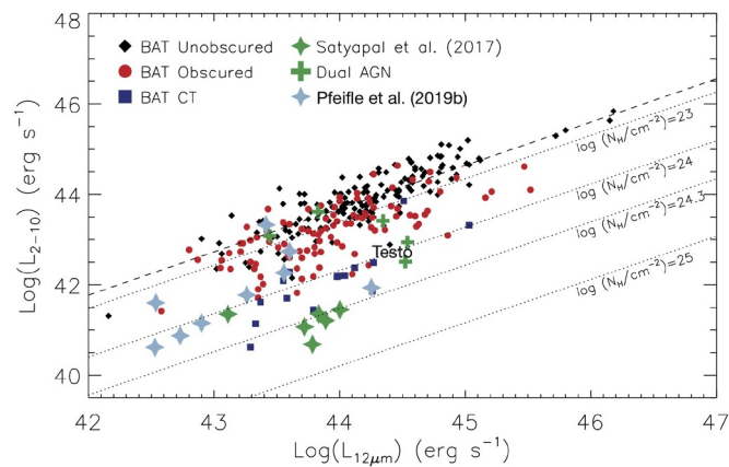
Fig. 4. 2–10 keV observed luminosity vs mid-IR (12 \mu\text{m} ) luminosity for the mergers included in the program described in Section 3.3 (i.e., X-ray follow-ups of WISE-selected mergers). The plot also includes the sources already confirmed as dual AGN in the literature. The samples of hard X-ray selected AGN with the Swift /BAT survey are also shown; for these AGN, a direct measurement of the absorbing column density N_{\text{H}} is possible (Ricci et al., 2015; 2017). The dual AGN candidates derived from the WISE selection are the most heavily absorbed. Dotted lines represent the effect of different absorption column densities on the unabsorbed best-fit linear relation from the Swift /BAT sample (dashed line). Adapted from (Pfeifle et al., 2019b).
