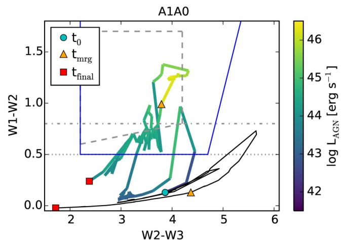
Fig. 14. Time evolution of the same merger shown in Fig. 13 in the WISE color-color space. The thick colored line refers to the fiducial analysis, whereas the thinner black line refers to the analysis not including any AGN component. The circles, triangles, and squares pinpoint the beginning of the run, the time of BH merger, and the end of the run, respectively. The horizontal lines refer to the commonly used thresholds for AGN selection ( W1-W2 > 0.5 and W1-W2 > 0.8 ). The gray dashed line refers to the two-color selection criterion proposed in Jarrett et al. (2011), whereas the blue solid line indicates the selection criterion proposed by Blecha et al. (2018). Adapted from Blecha et al. (2018). (For interpretation of the references to color in this figure legend, the reader is referred to the web version of this article.)
