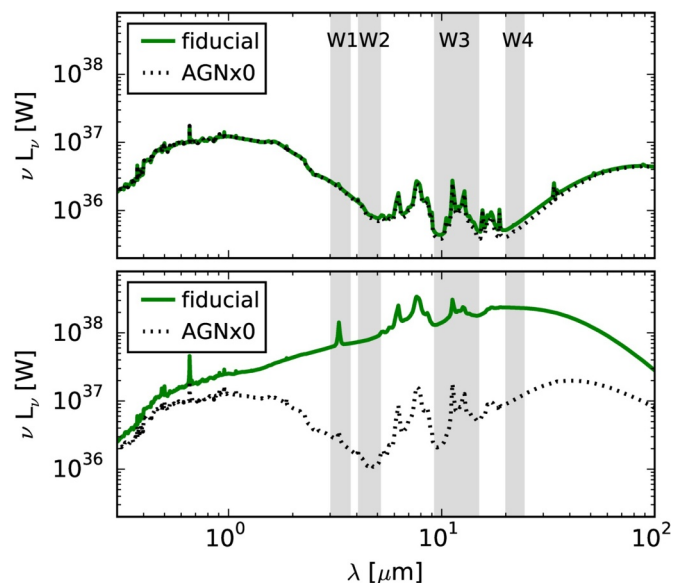
Fig. 13. Optical to IR SED of a 1:2 gas-rich merger in Blecha et al. (2018), the first time at which the separation between the two BHs drops below 10 kpc (upper panel), and immediately after the final pairing of the two BHs (lower panel). The solid line refers to the fiducial analysis, whereas the dotted line shows the SED obtained neglecting the input from any AGN activity. The shaded areas indicate the four WISE bands. Adapted from Blecha et al. (2018).
