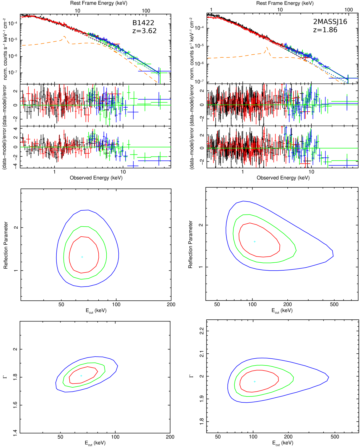
Figure 1. Top: Normalized spectra and residuals from the fit of B1422 (left) and 2MASSJ16 (right) with the phenomenological model. The lower panels show residuals from the fit with no high-energy cut-off. Black, red, green and blue points show XMM-Newton pn, MOS1+2, NuSTAR FPMA and FPMB data, respectively. Data binned for plotting purposes. The orange dashed lines show the reflection component. Center: Confidence contours, at 68, 90 and 99% c.l., of the reflection parameter R vs. E_{\text{cut}} . Bottom: Same for the photon index \Gamma vs. E_{\text{cut}} .
