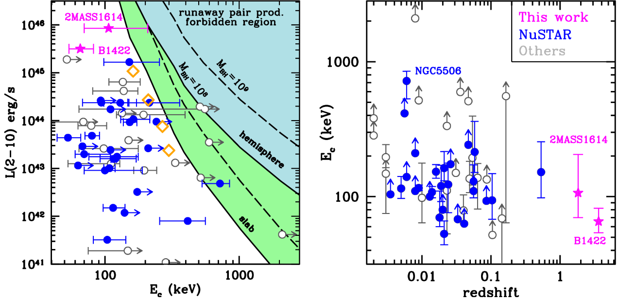
Figure 2. Left: E_{\text{cut}} vs. L_X for the updated F15 sample ( NuSTAR measurements in blue, non-focusing hard X-ray telescopes in gray). The two QSOs analyzed here are in magenta. The cyan (green) area shows the forbidden region due to runaway pair-production for an hemispheric (slab) corona for M_{\text{BH}} = 10^8 M_\odot . Dashed lines show the same limits for M_{\text{BH}} = 10^9 M_\odot . Orange diamonds show the results from the BAT AGN survey (Ricci et al. 2018). Right: E_{\text{cut}} vs. redshift for the same samples reported in the left panel.
