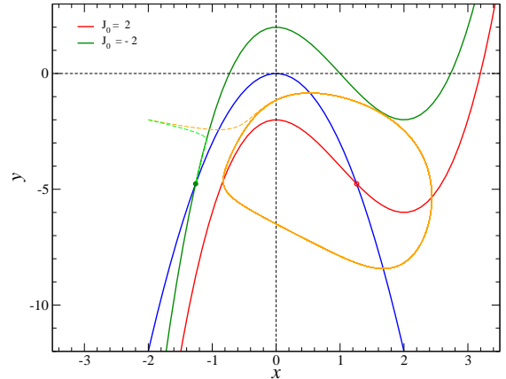
Figure 1. Nullclines for the system of Eq. 6 with \beta = 3 and for J_0 values equal to -2 (green curve) and 2 (red curve); the blue curve is the parabola given by the second formula of Eq. 7. Two phase trajectories (dashed lines) with the same initial conditions and corresponding to the two J_0 values are also shown: the green one moves along its nullcline to the stable equilibrium point (green filled circle) while the orange line describes a closed orbit around the unstable equilibrium point (red open circle).
