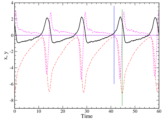
Figure 7. Numerical solutions of the variable y(t) (red curve) and its first derivative (magenta curve) compared with the x(t) (black curve) when in the \rho spiking class. The blue and green vertical lines limit the interval between a maximum and a minimum of y(t) where it is very quickly decreasing that corresponds to the highest emission in the x(t) peak. The violet horizontal line marks the zero level.
