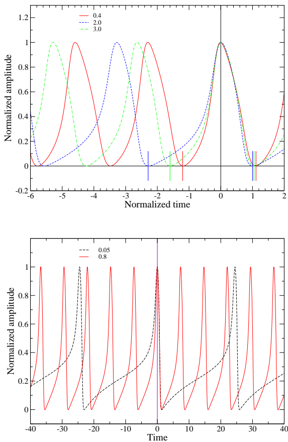
Figure 8. Upper plot: Normalized profiles of three spikes of the \rho class obtained by the MHR model for three values of J_0 without the random component. Vertical bars mark the initial and final points of the corresponding colour spikes. Curves, after the subtraction of the minimum level, are normalized in amplitude by taking the maximum value equal to unity, and in time by fixing to 1.0 the duration of the interval between the maximum and the end point of the spike for J_0 = 2.0 (blue line).
