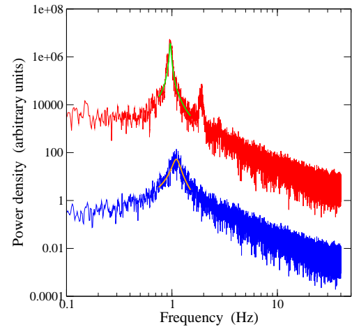
Figure 12. Upper plot: Light curves computed applying the MHR mathematical model assuming J(t) of Eq. 8, with C = 3.5 and two values of J_0 = 6.1 (red curve), just higher than the transition level and 7.5 (blue curve), both located in the stable region. Lower plot: power density spectra of these curves, shifted to separate the profiles of QPO features. The green and oranges thick curves are the Lorentzian fits of the QPO peaks.
