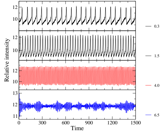
Figure 10. Light curves computed applying the MHR mathematical model assuming J(t) of Eq. 8, with C = 3.5 and different J_0 to change the position of the equilibrium point from the unstable to the stable region. The values of J_0 from top to bottom are 0.3, 1.5 ( \rho class), 4.0 (hfo), 6.5 (QPO).
