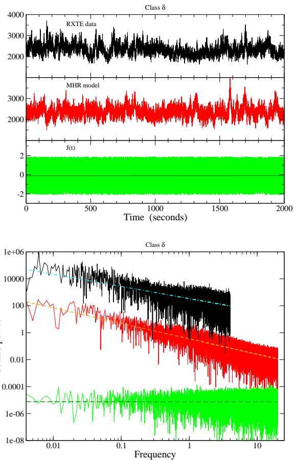
Figure 4. Upper plot: segment of a RXTE/PCA light curve of the \delta class (ID 10408-01-13-00) in the 2-12 keV energy interval (black curve in the top panel); light curve obtained by means of the MHR model (red curve in the central panel) using as input function the green curve in the bottom panel obtained by the superposition of a white random noise C = 4.0 to a constant level J_0 = -0.1 ; the mean value is represented by the dark green horizontal line.
