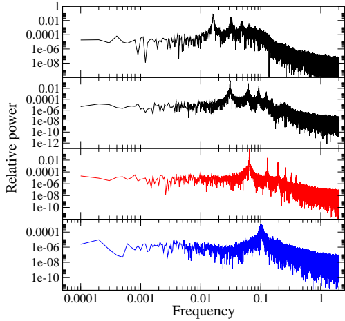
Figure 11. Power density spectra of the light curves in Fig.10. The two upper panels correspond to the spiking of the \rho class, while the third panel (red curve) is that of the ‘hfo’. All these spectra are dominated by the narrow lines and their harmonics of the periodic signals. The blue spectrum in the last panel has a unique broad peak typical of a QPO.
