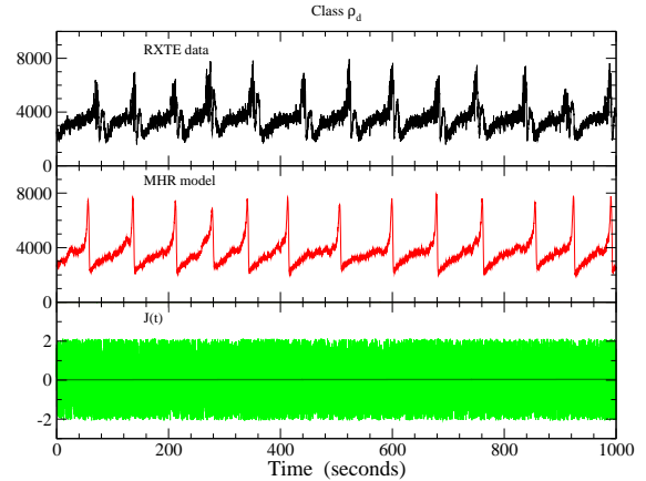
Figure 6. Top: segment of a RXTE/PCA light curve of the \rho_d class of the observation ID 10408-01-41-00 in the 2-12 keV energy interval. Central: light curve (red) obtained with the MHR model using the input model in the bottom panel. Bottom: input function J(t) with random fluctuations obtained with C = 4.0 superposed to a constant value J_0 = 0.05 ; its mean value is the dark green line.
