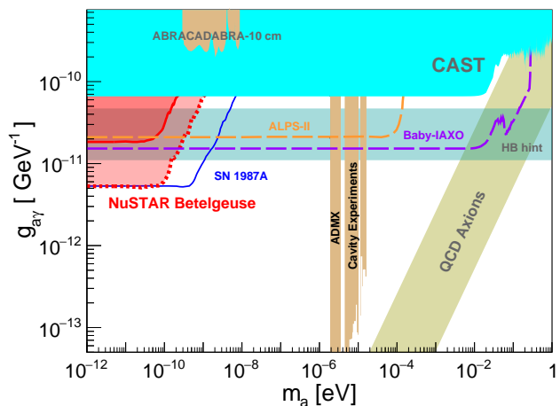
FIG. 3. Comparison of 95% upper limits of g_{a\gamma} from NuSTAR Betelgeuse observation is shown in red band: upper solid line for the most conservative stellar model and B_T , lower dashed line for the most optimistic stellar model and B_T , and the interval for the other combinations. Overlaid are the region of interest for QCD axion [47], the current limits from CAST [10], ADMX [46], ABRACADABRA-10cm [45] and SN 1987A [11], the projected sensitivity of ALPS-II [22] and Baby-IAXO [23, 24]. Also labelled are the ALP regions suggested by hints of excess gamma-ray transparency or cooling of horizontal-branch stars [48, 49].
