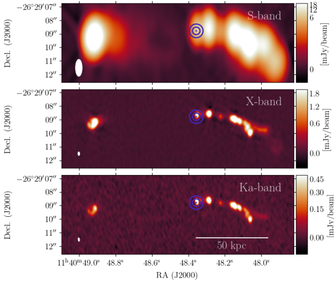
FIG. 1.— Multi-frequency synthesis maps of the Spiderweb radio jet and lobes at S-band (row a ), X-band (row b ), and Ka-band (row c ). The full source is shown for scale and perspective. All maps are shown on the same coordinate scale. The X- and Ka-band images are presented with square-root-stretched color scales. The S-band image is presented with a logarithmic color scale to emphasize detail over a larger dynamic range. For all images, the sensitivity is approximately 5 \mu\text{Jy}/\text{beam} . The synthesized beam areas are indicated at the bottom-left in the right-hand column of plots. The position of the X-ray AGN core (Tozzi et al. 2022) is indicated with blue concentric circles. The angular scale is identical between images; the white scale-bar indicates a projected span of 50 kpc at z = 2.16 for the adopted cosmology.
