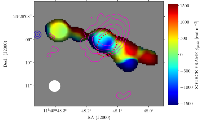
FIG. 4.— Colorscale: Hue-intensity map of the western radio jet. The hue channel traces source-frame RM, while the intensity channel traces peak- P . The color map has been selected to highlight local differences in RM. Masking is the same as Figure 2. A flat Galactic foreground contribution of -13 \text{ rad m}^{-2} has been subtracted from \phi_{\text{peak}} (Hutschenreuter & Enßlin 2020). Contours: Lyman- \alpha emission. Levels start at 35 arbitrary units, and increase by a factor of \sqrt{2} . The red dotted line indicates the location of the RM enhancement discussed in the main text. The position of the X-ray AGN core (Tozzi et al. 2022) is indicated with blue concentric circles. The white filled circle indicates the effective synthesized beam size.
