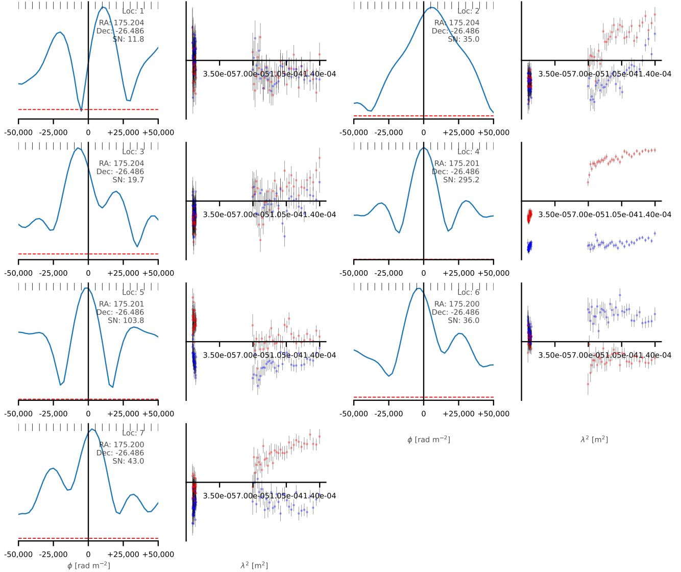
FIG. 3.— The calculated dirty (i.e. no rmclean performed; Heald et al. 2009) FDS (first & third columns) and corresponding Stokes Q (red) and U (blue) spectra (second & fourth columns) for the seven high- |RM| locations labeled in Figure 2 panel (b), and listed in Table 2. For the FDS plots, the horizontal axes range from -50,000 to +50,000 \text{rad m}^{-2} in the source frame. The gray minor tick marks at the top of each panel indicate increments of 5,000 \text{rad m}^{-2} . For the QU plots, the horizontal axes span 0 – 1.4 \times 10^{-4} \text{m}^2 , again in the source frame. The vertical axes limits are all scaled to the maximum amplitude of the data points in individual plots. The location number (corresponding to those shown in Figure 2 panel (b) and Table 2), the right ascension, declination, and band-averaged polarized signal-to-noise ratio (SN) are all written in the respective FDS plots. The error bars on the (Q, U) data points indicate the standard deviation measured per image channel from the Stokes (Q, U) datacubes in a small region adjacent to each source. Note that because the FDS have not been deconvolved with rmclean , the emission-free regions of the FDS cannot be used as a guide to the underlying noise level. Note that the broad FDS peak seen at ‘location 2’ may be a rare example (see Section 3) where emission comes from a range of Faraday depths (i.e. shows ‘Faraday complexity’). This is unsurprising, given its location near RM ‘interfaces’ in the eastern hotspot complex.
