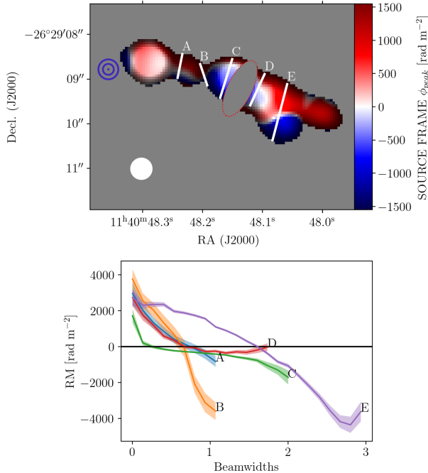
Fig. 5.— Top panel : Hue (source-frame RM)-intensity (peak- P ) map of western radio jet, as for Figure 4. A divergent color map has been selected to highlight areas where RMs are zero \text{rad m}^{-2} (white), positive (red) and negative (blue). Masking is the same as Figure 2, with the addition of a red-dotted ellipse, which also masks the peak- P enhancement attributed to local interaction with the \text{Ly}\alpha knot (described in Section 4.2.3). This emphasizes the surrounding global RM structure of the jet. Five cross sections running across the axis of the western jet, and spaced roughly equidistantly along the jet, are indicated by white lines and lettered designations. The location of the X-ray AGN core (Tozzi et al. 2022) is indicated with blue concentric circles. The white filled circle indicates the effective synthesized beam size. Bottom panel : Values of source-frame RM (colored lines) and their uncertainty (shaded regions), plotted as a function of angular distance in units of synthesized beamwidths, extracted from north to south along the cross-sections indicated by the corresponding letter designations in the top panel.
