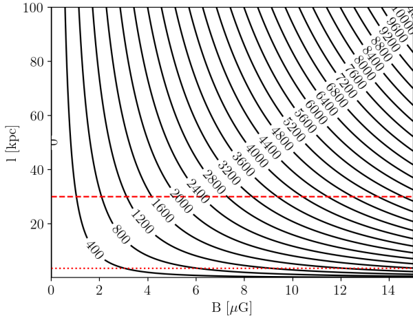
FIG. 7.— Contour plot showing values of \sigma_{\text{RM}} (in units of \text{rad m}^{-2} , in the source frame) as a function of the magnetic field strength B and turbulent length scale l , derived from Equation 4 using fixed values of n_e = 1.5 \times 10^{-2} \text{ cm}^{-3} and D = 100 \text{ kpc} . The numbers on the contours are \sigma_{\text{RM}} values in \text{rad m}^{-2} . The red dotted line is the FWHM of the common-resolution synthesized beam ( 0.5'' ) at the distance of the cluster. The red dashed line is the approximate radial extent of the radio jets in the cluster gas.
