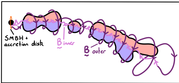
Fig. 6.— Toy model of the western jet (black outline), indicating how an RM gradient crossing from negative RMs (blue shading) to positive RMs (red shading; similar to Figure 5) across the jet axis could arise from a toroidal magnetic field component which is clockwise when viewed from the central SMBH and accretion disk (labelled). The picture is of a nested helix configuration, with inner and outer magnetic field windings (labelled), as discussed in Section 6).
