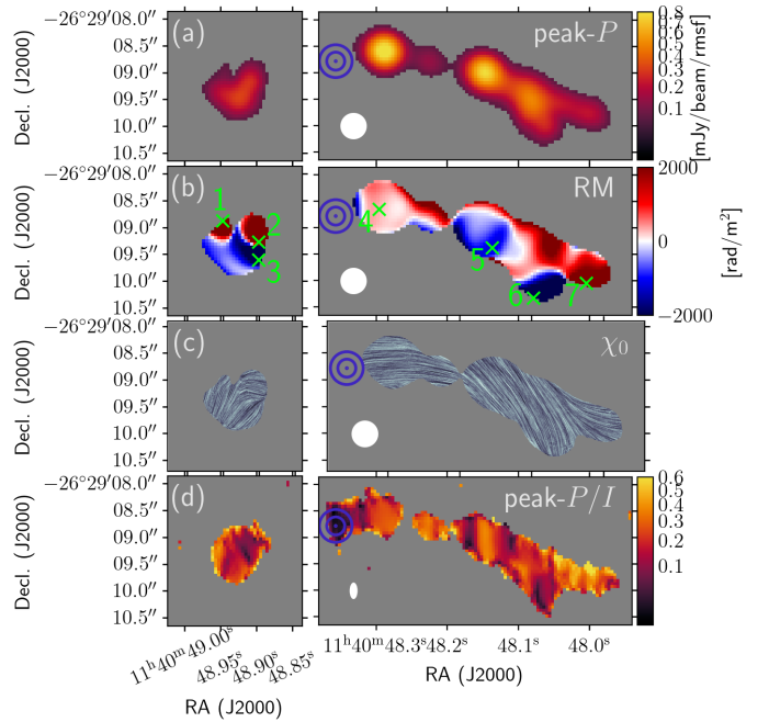
FIG. 2.— Maps of peak- P (X- plus Ka-band), source-frame RM (X- plus Ka-band; note that values saturate at \text{RM} = \pm 2000 \text{rad m}^{-2} to better reveal low |\text{RM}| structure throughout the jet), intrinsic sky-projected magnetic field orientation (Ka-band only), and fractional polarization (Ka-band only) across the Spiderweb radio jet (rows a – d respectively). The eastern and western jet components (see Figure 1) are shown in the left-hand and right-hand columns respectively. Coordinates are shared between axes in the same way as for Figure 1. The effective synthesized beam areas (see Section 3) are shown in the lower-left corner of the right-hand column of panels in white. The location of the X-ray AGN core (Tozzi et al. 2022) is indicated with blue concentric circles. The maps have been masked at full-band polarized signal-to-noise levels of 7\sigma (for their respective frequency band coverage). The map of fractional polarization has been masked at a full-Ka-band signal-to-noise of 10\sigma in the total intensity. The green ‘x’ markers on the RM map mark the positions at which RMs were extracted for values presented in Table 2. The uncertainties in RM (row b ), intrinsic magnetic field orientation (row c ), and fractional polarization (row d ) typically lie in the range 100–400 \text{rad m}^{-2} , 0–5 degrees, and 0–0.03, respectively.
