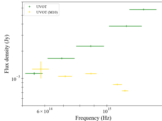
Figure 1. Comparison between the unabsorbed UVOT data in Migliari et al. (2010) (yellow points) and the unabsorbed UVOT data used in this paper (green points). In particular, for the new UVOT data set we corrected for an absorption coefficient of A_V \sim 1.5 , found using the model REDDEN on XSPEC (see subsection 4.2-4.3 for further details).
