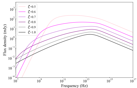
Figure 4. Simulated SEDs with ISHEM using several values of \zeta , from 1.0 to 0.5, without rescaling or shift factors applied, showing the impact of geometry on the flux and the shape of the emitted jet spectrum. In order to simulate these spectra, the X-ray PDS was used as input.
