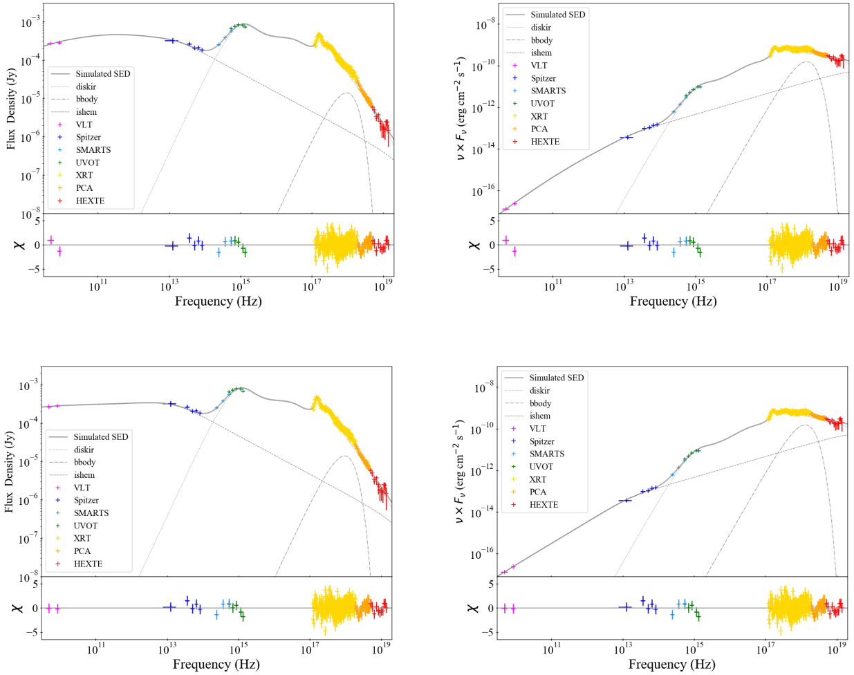
Figure 9. Best-fit unabsorbed spectral energy distribution compared with the whole multiwavelength dataset available for 4U 0614+091, in both Flux Density ( Left ) and \nu \times F_\nu ( Right ) representation. The optical-to-X-ray data set has been analysed with an irradiated disk + black-body model, while the radio-to-IR data set was modeled with ISHEM. In this plot we show both best-fit ISHEM models found in this paper: on Top the model built with the X-ray PDS and corresponding to a non-conical geometry ( \zeta = 0.6 ) and on ( bottom ) the model corresponding to a "flicker noise" PDS in conical geometry.
