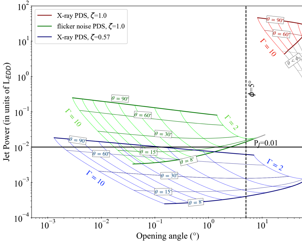
Figure 10. Jet power - (observed) opening angles curve (from Equations 1-2) for a different combinations of \zeta and PDS to a range of possible values for the inclination \theta and a range of \Gamma_{av} between 2 and 10. In particular, in each "region" (identified by a specific color) the inclination increases going upwards, while the Lorentz factor increases going from right to left. Curves for specific fixed values of \Gamma and \theta are identified to help the eye. In each area, the sub-region for which the condition \theta > \phi_0 is not satisfied are colored in grey and have to be discarded, as the used scaling relations are no longer valid
