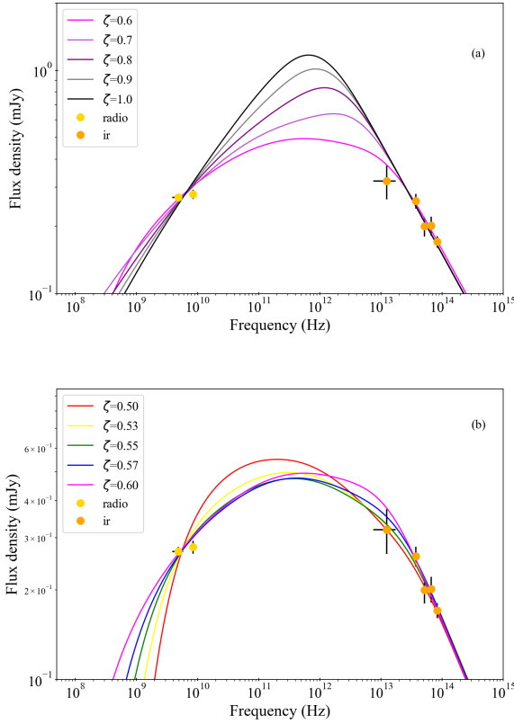
Figure 7. Simulated SEDs with ISHEM using several values of \zeta , from 1.0 to 0.6 (panel a ) and in the critical region 0.5 to 0.6 (panel b ), normalized and shifted in order to fit the data. In all these models, the X-ray PDS was used as an input for ISHEM. Panel b shows the interesting evolution of the SED for values of \zeta spanning in the crucial region between \zeta = 0.6 and \zeta = 0.5 : when the jet becomes too collimated, the contribution from the external regions of the jet (the lower frequencies) becomes dominant and it leads again to an inverted spectrum.
