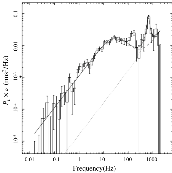
Figure 2. PDS in the normalized power ( P_\nu ) times frequency ( \nu ) representation, with the best fit multi-Lorentzian model.
