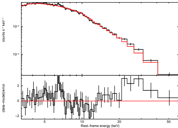
Fig. 2. Comparison of the data (black) and power law model (red). An excess of photons is observed between 6.4 and 7 keV suggesting the presence of emission features ascribable to neutral and/or possibly ionized iron. Also a bump of unmodelled photons is found above \sim 10 keV. For plotting purposes the FPMA and FPMB spectra of all the epochs and their residuals in terms of errors with respect to the model are displayed grouped ( setplot group in Xspec ).
