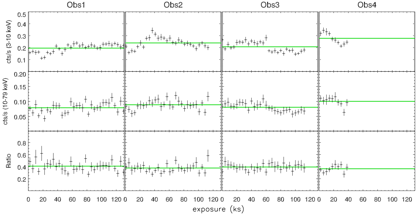
Fig. 1. Top and middle panels: coadded FPMA and FPMB light curves shown in the 3–10 keV and 10–79 keV energy bands, respectively. For the various pointings, the ratios between the 10–79 keV light curves and those computed in the 3–10 keV band are shown. The adopted time binning is 4 ks for all the observations. Solid green lines account for the average count rates within each pointing. The exposures in the graph are twice as long as those reported in Table 1 because half of the NuSTAR time is cut due to Earth occultations.
