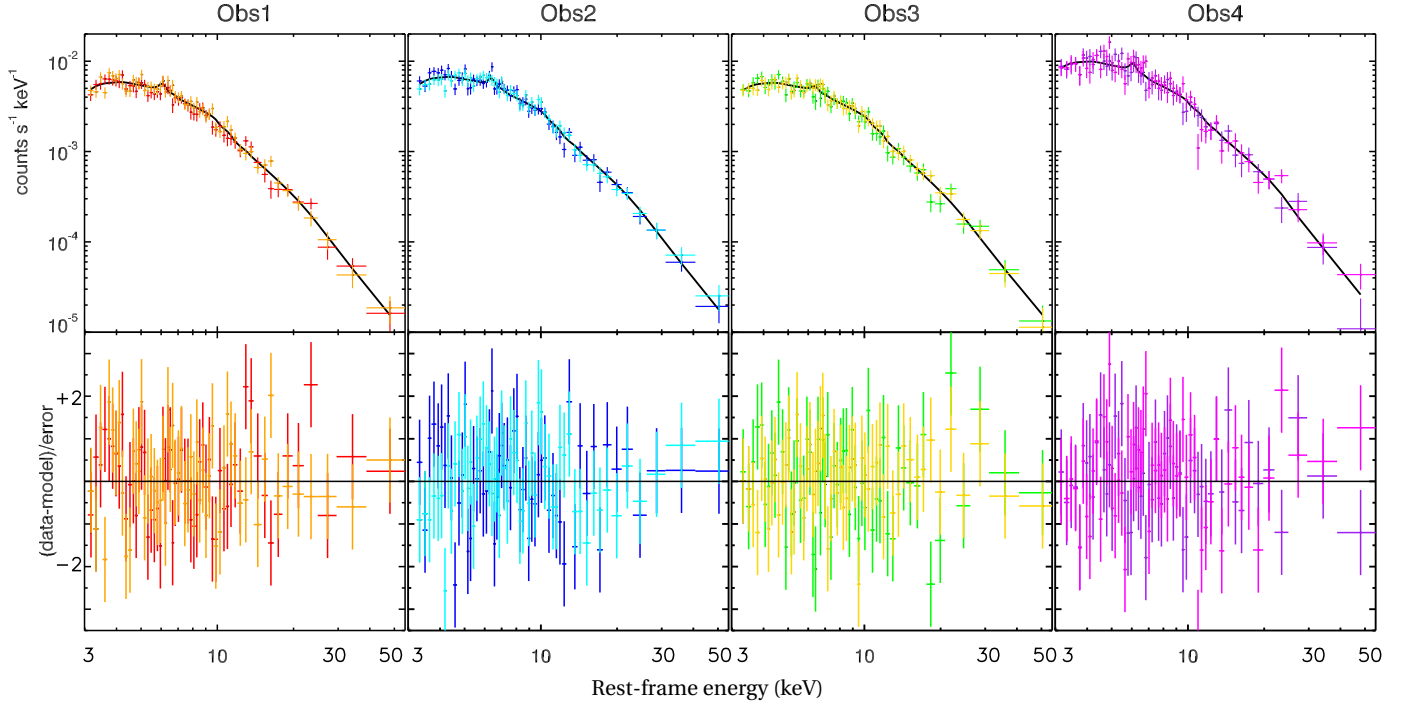
Fig. 3. Best-fit model const. \times phabs \times xillver to the NuSTAR data displayed for each observation. In the x -axis the energy is reported in keV and different colours are used to represent the NuSTAR module A and B spectra.
