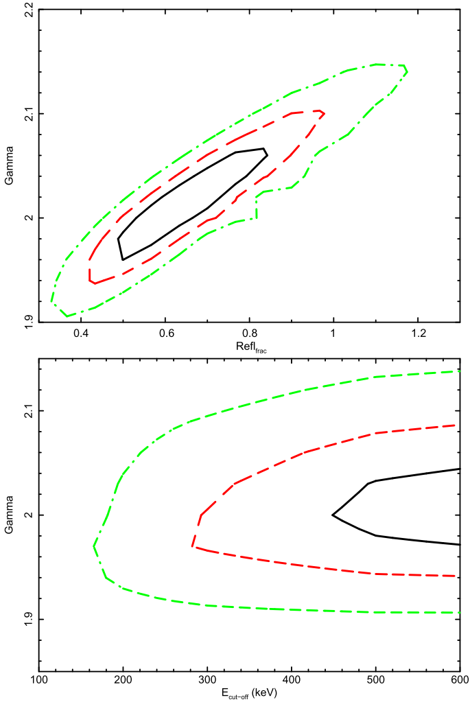
Fig. 4. The 68%, 90% and 99% contours in black, red, green respectively computed adopting const. × phabs × xillver . Top panel: photon index and reflection fraction. Bottom panel: contours for the photon index and the high energy cut-off.
