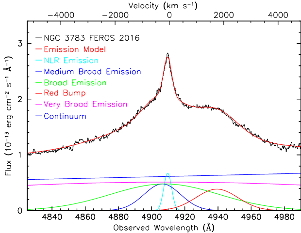
Fig. 19. FEROS spectrum of the H \beta region from observations in 2016 December (black histogram). The solid red line tracing the data is the total emission model. The key in the figure identifies the emission components in our model. The velocity scale along the top axis is for the rest wavelength of H \beta relative to the host galaxy systemic redshift, z = 0.00973 (Theureau et al. 1998).
