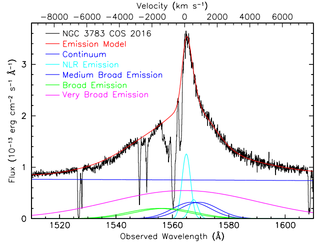
Fig. 12. Best fit with no absorption to the average COS spectrum of the C IV region from observations in 2016 December. The black histogram shows the data. The solid red line tracing the data is the total emission model. The key in the figure identifies the emission components in our model. The velocity scale along the top axis is for the blue component of the C IV doublet, \lambda 1548.195 , relative to the host galaxy systemic redshift, z = 0.00973 (Theureau et al. 1998).
