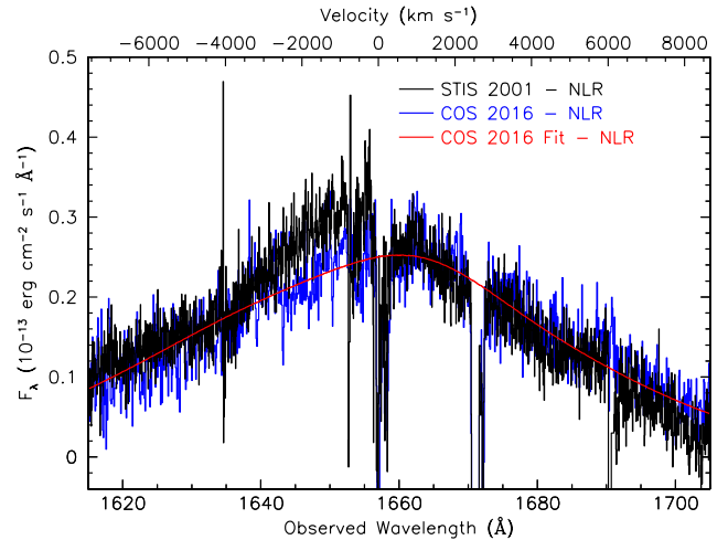
Fig. 7. Comparison of STIS and COS spectra of the region surrounding the He II emission line omitting the narrow emission. The black histogram shows the average STIS 2001 spectrum with the narrow components of He II and O III] subtracted. The blue histogram shows the unweighted average COS spectrum from the 12 December 2016 and 21 December 2016 observations, also with the narrow components subtracted. Both spectra have the continuum subtracted as well as the underlying emission of the C IV emission line. The STIS spectrum is scaled up 1.2\times to match the flux in the far wings of the COS spectrum. The solid red line represents the best-fit emission model for the COS spectrum. The velocity scale along the top axis has zero velocity for He II \lambda 1640.45 at the host-galaxy redshift of 0.00973 (Theureau et al. 1998).
