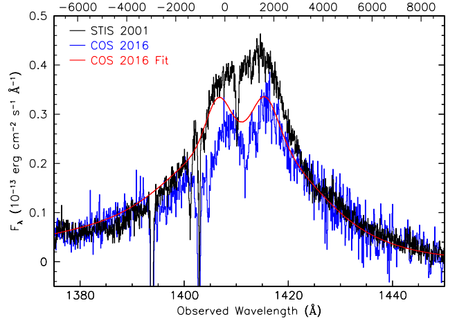
Fig. 14. Comparison of STIS and COS spectra surrounding the region of the Si iv emission line. The black histogram shows the average STIS 2001 spectrum. The blue histogram is the unweighted average COS spectrum from 2016. The solid red line is the best-fit emission model for the COS spectrum. The velocity scale along the top axis is for Si iv \lambda 1393.755, relative to the host galaxy systemic redshift, z = 0.00973 (Theureau et al. 1998).
