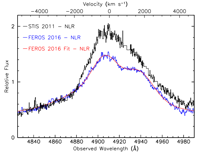
Fig. 18. FEROS (blue) and STIS (black) spectra of the H\beta region with the continuum and narrow H\beta emission component subtracted from each. The FEROS spectrum has been scaled to match the STIS spectrum in the far blue wing of the emission-line. The solid red line tracing the data shows the total emission model with the continuum and narrow emission component subtracted. The velocity scale along the top axis is for the rest wavelength of H\beta relative to the host galaxy systemic redshift, z = 0.00973 (Theureau et al. 1998).
