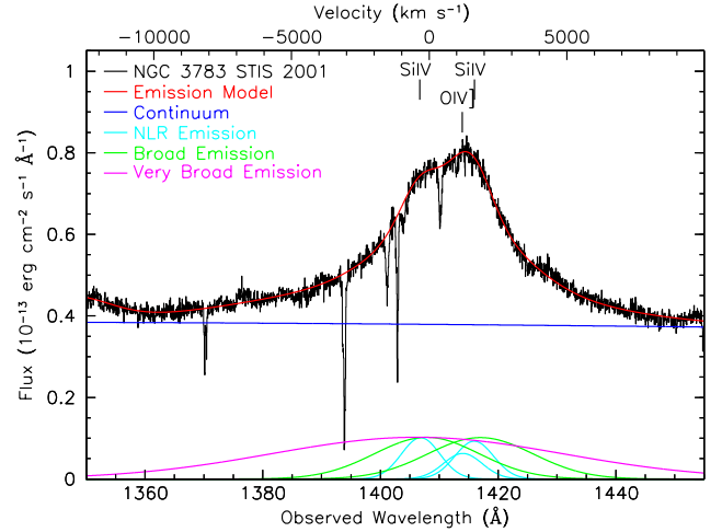
Fig. 4. Average STIS spectrum of the Si iv region from all observations in the 2000–2001 campaign re-binned into 0.05 Å pixels (black histogram). The solid red line tracing the data shows the total emission model. The key in the figure identifies the emission components in our model. The velocity scale along the top axis is for Si iv \lambda 1393.755, relative to the host galaxy systemic redshift, z = 0.00973 (Theureau et al. 1998).
