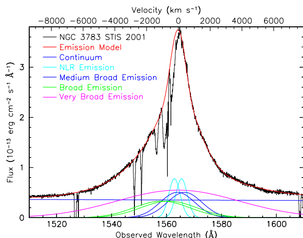
Fig. 2. Average STIS spectrum of the C iv region from all observations in the 2000–2001 campaign re-binned into 0.05 \text{ \AA} pixels (black histogram). The solid red line tracing the data shows the total emission model. The key in the figure identifies the emission components in our model. The velocity scale along the top axis is for the blue component of the C iv doublet, \lambda 1548.195 , relative to the host galaxy systemic redshift, z = 0.00973 (Theureau et al. 1998).
