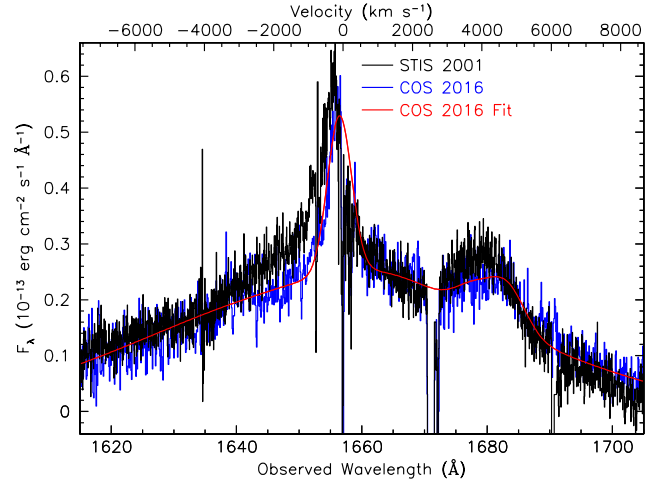
Fig. 6. Comparison of STIS and COS spectra of the region surrounding the He II emission line. The black histogram shows the average STIS 2001 spectrum. The blue histogram shows the unweighted average COS spectrum from the 12 December 2016 and 21 December 2016 observations. Both spectra have the continuum subtracted as well as the underlying emission of the C IV emission line. The STIS spectrum is scaled up by 1.2\times to match the flux in the far wings of the COS spectrum. The solid red line is the best-fit emission model for the COS spectrum. The velocity scale along the top axis has zero velocity for He II \lambda 1640.45 at the host-galaxy redshift of 0.00973 (Theureau et al. 1998). All narrow absorption features are foreground ISM lines.
