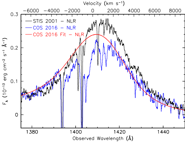
Fig. 16. Spectra of the Si IV region as in Fig. 15, but with both the STIS and the COS spectra smoothed by a seven-pixel running boxcar filter. The solid red line is the best-fit emission model for the COS spectrum minus the narrow emission components. The velocity scale along the top axis is for Si IV \lambda 1393.755, relative to the host galaxy systemic redshift, z = 0.00973 (Theureau et al. 1998).
