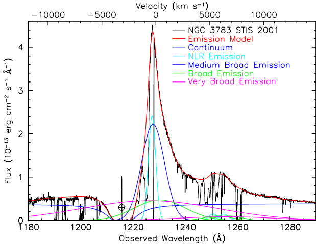
Fig. 3. Average STIS spectrum of the Ly \alpha +N v region from all observations in the 2000–2001 campaign re-binned into 0.05 Å pixels (black histogram). The solid red line tracing the data shows the total emission model. The key in the figure identifies the emission components in our model. The velocity scale along the top axis is for Ly \alpha \lambda 1215.67, relative to the host galaxy systemic redshift, z = 0.00973 (Theureau et al. 1998). Geocoronal emission in the center of the Milky Way Ly \alpha absorption trough is indicated with an Earth symbol. The solid blue line showing the continuum also illustrates the impact of the damped Milky Way Ly \alpha absorption. We note that the influence of this damping profile extends all the way from 1180 Å on through the peak of Ly \alpha in NGC 3783 and into the N v profile at 1250 Å.
