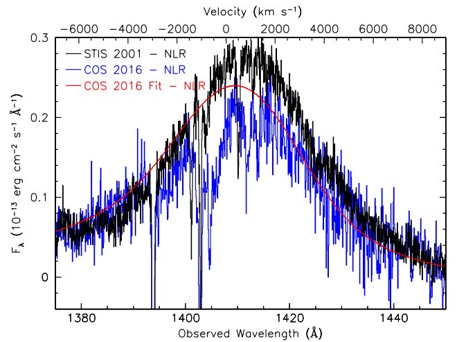
Fig. 15. Comparison of STIS and COS spectra of the region surrounding the Si iv emission line omitting the narrow emission components. The black histogram shows the average STIS 2001 spectrum with the narrow emission components of Si iv and O iv] subtracted. The blue histogram is the unweighted average COS spectrum from 2016, also with the narrow emission components subtracted. The solid red line is the best-fit emission model for the COS spectrum minus the narrow emission components. The velocity scale along the top axis is for Si iv \lambda 1393.755, relative to the host galaxy systemic redshift, z = 0.00973 (Theureau et al. 1998).
