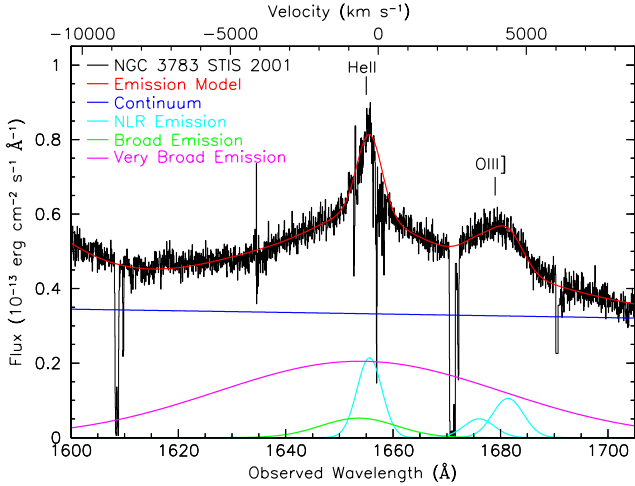
Fig. 5. Average STIS spectrum of the He II region from all observations in the 2000–2001 campaign re-binned into 0.05 \text{ \AA} pixels (black histogram). The solid red line tracing the data show the total emission model. The key in the figure identifies the emission components in our model. The velocity scale along the top axis is for He II \lambda 1640.45 , relative to the host galaxy systemic redshift, z = 0.00973 (Theureau et al. 1998). All narrow absorption features are foreground ISM lines.
