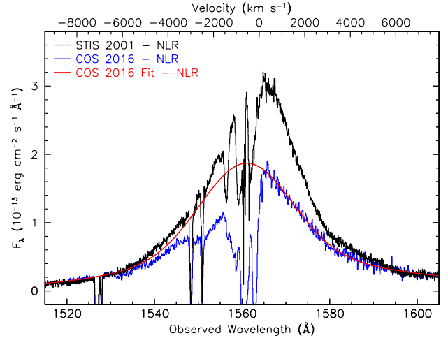
Fig. 9. Average STIS spectrum of the C IV region from all observations in the 2000–2001 campaign re-binned into 0.05 \text{ \AA} pixels (black histogram) with the narrow-line component of the fit subtracted from the data. The blue histogram shows the average COS spectrum from 2016 with the narrow-line component subtracted. The STIS data have been scaled up by a factor of 1.45 so that the intensities match in the broad wings. The solid red line tracing the data is the total emission model for the average 2016 COS spectrum with the narrow-line component removed. The velocity scale along the top axis is for C IV \lambda 1548.195 , relative to the host galaxy systemic redshift, z = 0.00973 (Theureau et al. 1998).
