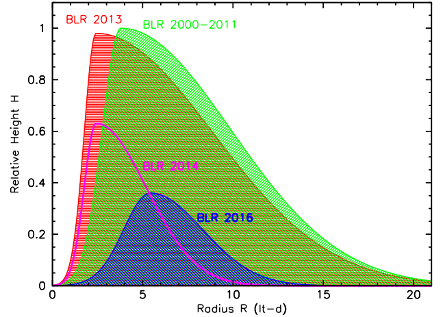
Fig. 29. Schematic representation of the evolution of the BLR in NGC 3783. The green shaded area represents the vertical structure and radial extent of the BLR during the period from 2000 to 2011. The red shaded area shows the inferred structure in 2013, when the continuum flux was 2.5 \times less, but the EW of C IV was 70% higher. The magenta curve is the hypothetical structure in 2014, when the continuum flux was still low after the BLR had dynamically adjusted to the lower flux level. The blue shaded area is the inferred structure at the time of the obscuration event in 2016.
