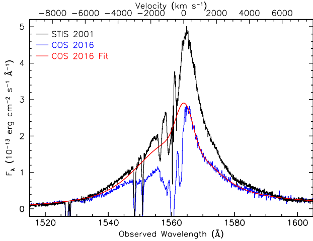
Fig. 8. Average STIS spectrum of the C IV region from all observations in the 2000–2001 campaign re-binned into 0.05 \text{ \AA} pixels (black histogram). The blue histogram shows the average COS spectrum from 2016. The STIS data have been scaled up by a factor of 1.45 so that the intensities match in the broad wings. The solid red line tracing the data is the total emission model for the average 2016 COS spectrum. The velocity scale along the top axis is for C IV \lambda 1548.195 , relative to the host galaxy systemic redshift, z = 0.00973 (Theureau et al. 1998).
