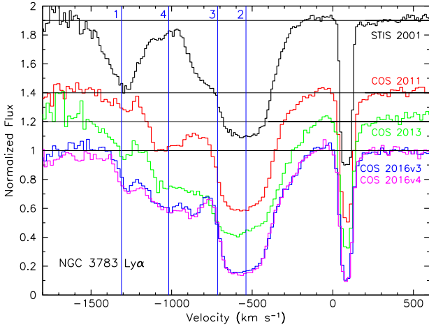
Fig. 22. Normalized HST spectra of the Ly \alpha region from five different epochs as labeled. Velocity is for Ly \alpha \lambda 1215.67 relative to the host galaxy systemic redshift of z = 0.00973 (Theureau et al. 1998). Fluxes are normalized to range from 0 to 1. Epochs prior to 2016 are offset vertically by 0.2, 0.4, and 0.9, with the offset normalizations indicated by thin horizontal black lines. The velocities of Components 1–4 as given by Gabel et al. (2003b) are marked by thin vertical blue lines and labeled.
