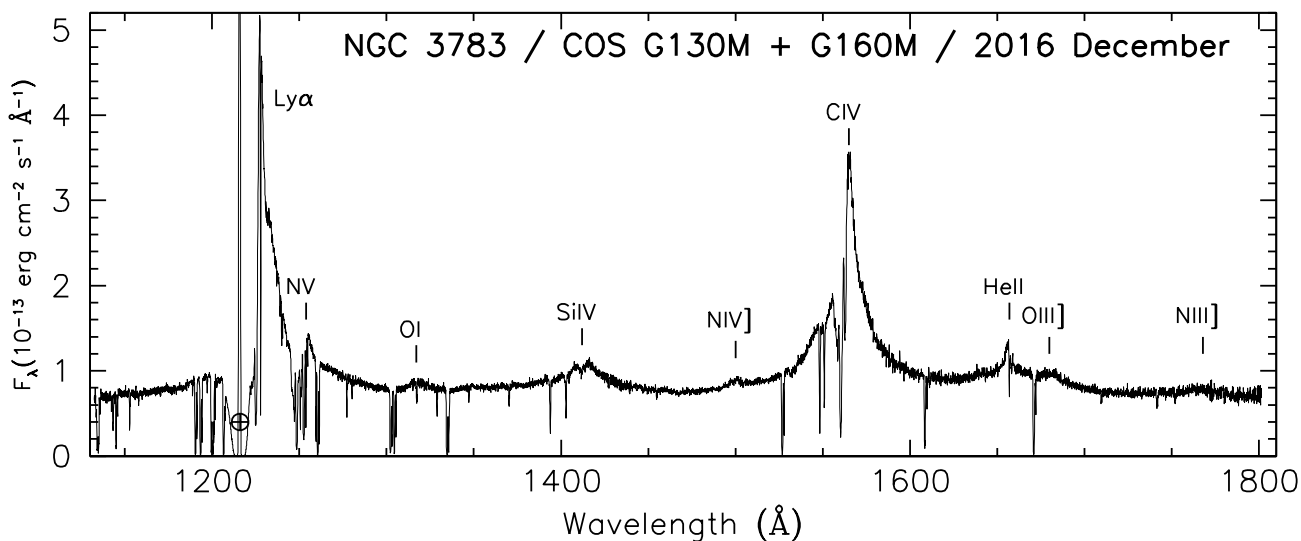
Fig. 1. Calibrated and merged COS spectrum of NGC 3783 from 2016 December. Data are binned by eight pixels, or approximately one resolution element. We label the most prominent emission features. Geocoronal emission in the center of the Milky Way Ly \alpha absorption trough is indicated with an Earth symbol.
