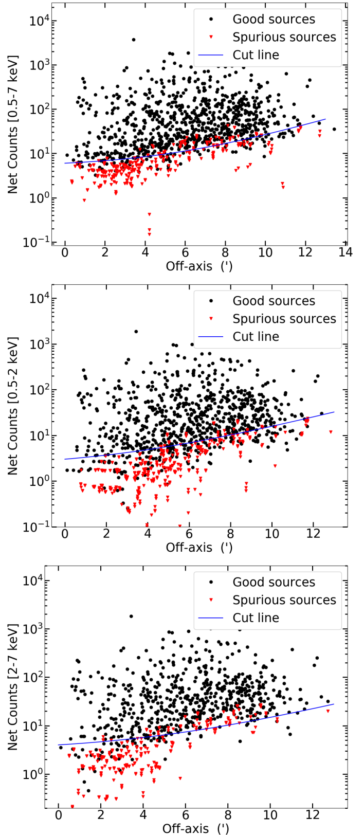
Fig. 6. Net counts vs. off-axis angles for the sources detected in the three simulations in the full ( top ), soft ( middle ), and hard ( bottom ) bands. The black dots are the “good” input–output matches according to the likelihood-ratio method, while the red triangles are those considered as spurious. The blue line represents the source-count limit as a function of the off-axis angle adopted to compute the completeness and reliability.
