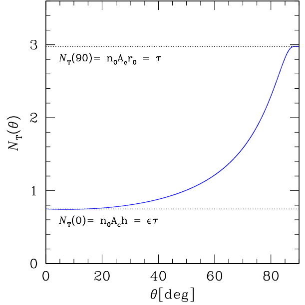
Fig. 7. Variation of the average number of ISM clouds along a given line of sight to the nucleus as a function of the viewing angle \theta ( 90^\circ is edge on) for a typical massive galaxy with M_{gas} \sim 10^{10} M_\odot at z = 2.5 .
