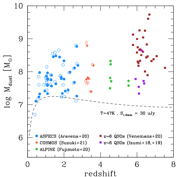
Fig. 1. Estimated dust mass vs. redshift for the considered galaxy samples as labeled. For high- z QSO hosts, dust masses have been estimated from Eq. 2 assuming T_d=47 K if T_{min} < 47 K or T_d = 1.2T_{min} if T_{min} > 47 K (see text for details). For the ASPECS and COSMOS samples, the original dust masses derived through SED-fitting (MAGPHYS) are plotted as open symbols, and those derived from a single MBB with T_d = 47 K as filled symbols. The dashed curve shows the dust mass limit corresponding to a flux density of 30 \mu Jy at 1.2 mm (i.e., the \sim 3\sigma detection limit in ASPECS) from Eq. 2 assuming T_d=47 K.
