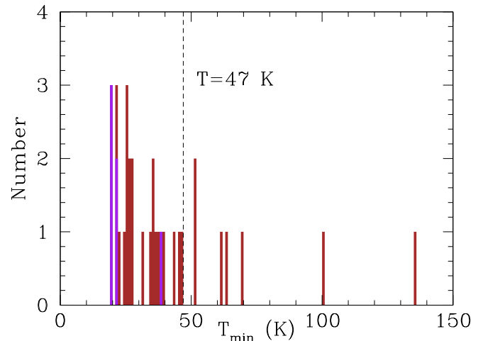
Fig. 3. Distribution of the minimum blackbody temperature T_{min} required to explain the observed 1.2 mm brightness of z \sim 6 QSOs. The Venemans et al. (2020) and SHELLQs samples are shown in brown and purple, respectively. Note that the 1.2 mm emission on approximately kiloparsec scales of a few bright objects can only be reproduced by hot dust with T_d > 50 - 100 K. We used T_d = 47 K, a standard reference value used in the literature (e.g., Venemans et al. 2020), to derive the dust masses of all QSOs with T_{min} < 47 K. For hotter systems, we used T_d = 1.2T_{min} (see text for details).
