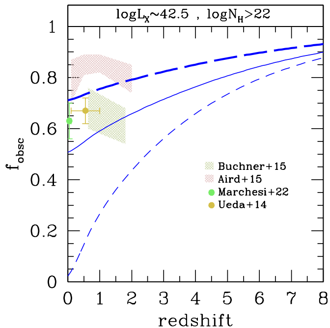
Fig. 15. Total fraction of obscured AGN with \log N_H > 22 vs redshift observed in different X-ray samples of low-luminosity AGN ( \log L_X \approx 42.5 ; see text for details). Model curves are as in Fig. 14. The model with \gamma = 2 and \theta_{\text{torus}} = 45^\circ (thick dashed blue line) provides a reasonable representation of the data.
