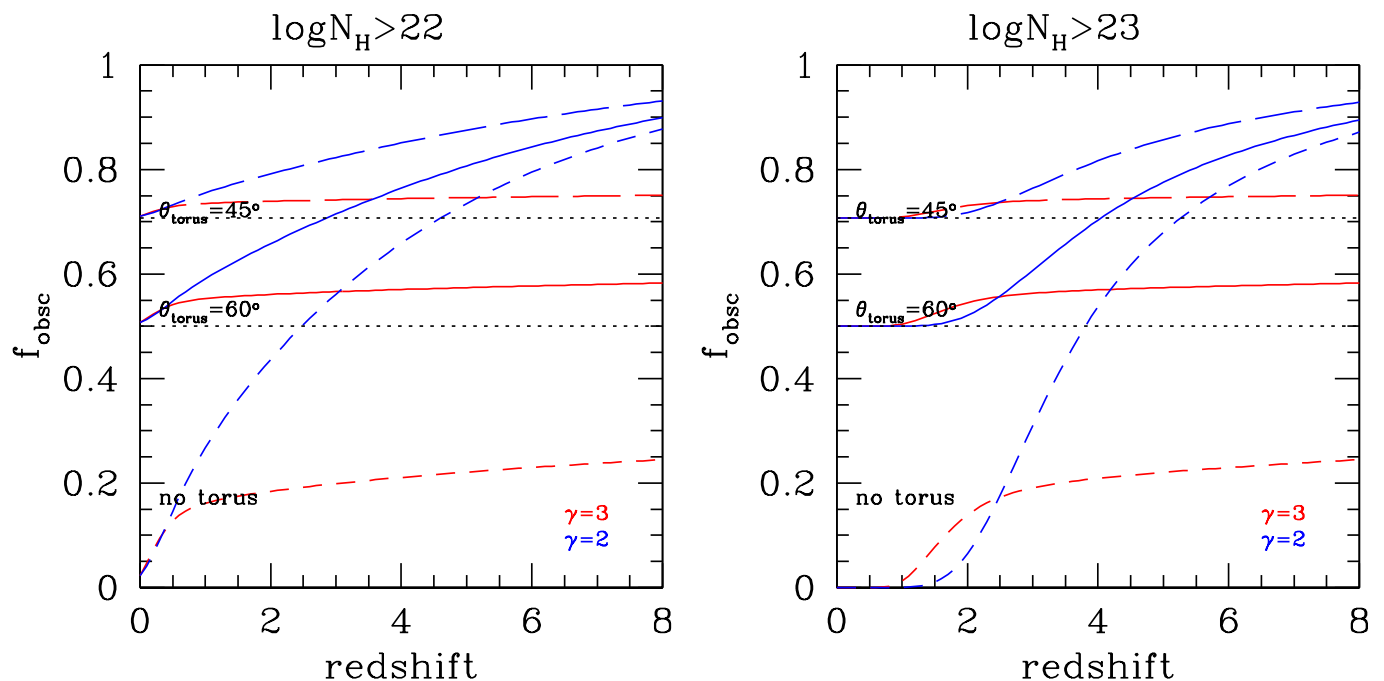
Fig. 13. Total fraction of obscured AGN with \log N_H > 22 (left panel) and \log N_H > 23 (right panel) vs. redshift for different combinations of large-scale (ISM) and small-scale (torus) obscuration. All curves are for \delta = 3.3 and \epsilon = 0.25 . The characteristic surface density \Sigma_{c,*} of ISM clouds is assumed to evolve as \propto (1+z)^\gamma , with \gamma = 2 (blue curves) or \gamma = 3 (red curves). Short dashed lines refer to ISM-only obscuration (i.e., no torus considered, as in Fig. 11). Long dashed and solid lines show the total obscured AGN fraction when adding a torus with half-opening angle \theta_{\text{torus}} = 45^\circ and 60^\circ , respectively. The horizontal dotted lines show the obscured AGN fraction expected by torus-only obscuration.
