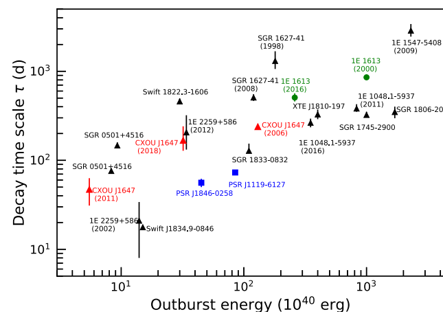
Figure 8. Decay time-scale (in terms of e-folding time) as a function of the total energy released for magnetars showing major outbursts. The triangles refer to the ‘canonical’ magnetars and in red we highlighted the 2006, 2011, and 2018 outbursts of CXOU J164710.2–455216. Blue squares indicate the rotation-powered pulsars with high magnetic fields that showed magnetar-like activity. The green circles denote the two outbursts of 1E 161348–5055, the central source of the supernova remnant RCW 103. Adapted from Coti Zelati et al. (2018).
