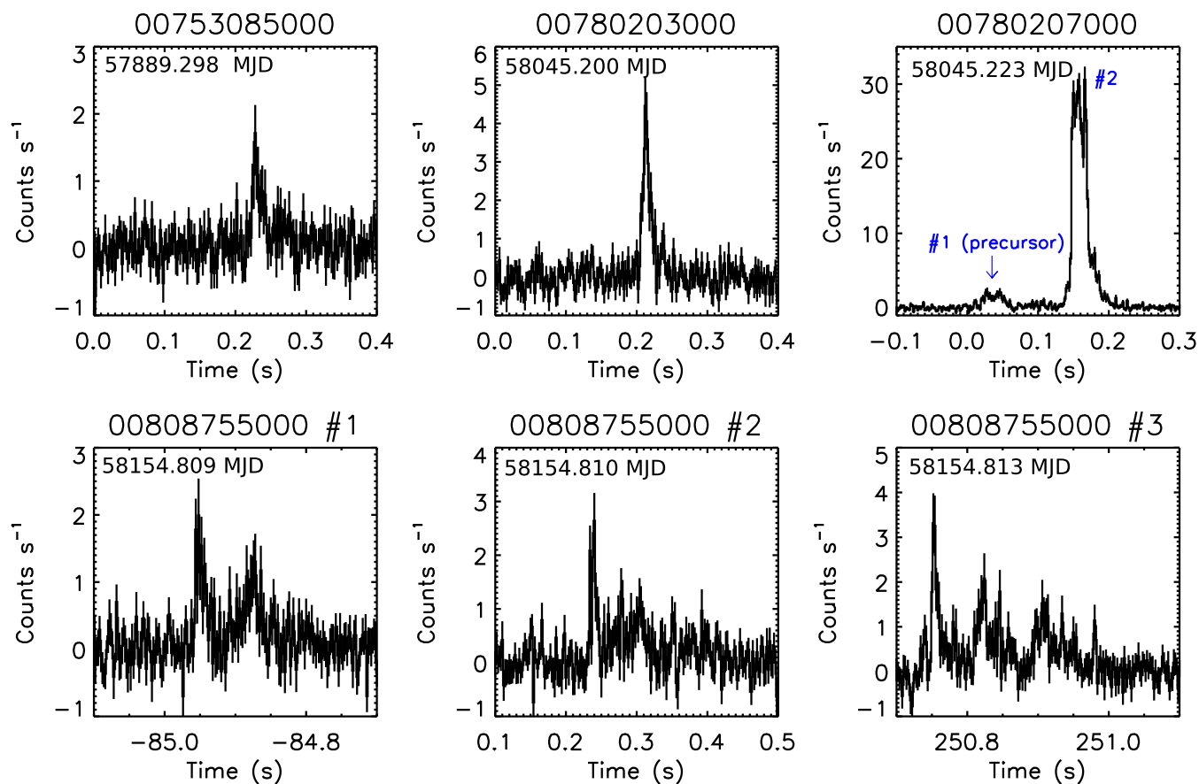
Figure 1. Light curves of the bright bursts detected from CXOU J164710.2–455216 with Swift BAT (as indicated in each panel). The energy range is 15–150 keV, the bin size 2 ms and the time is counted from the trigger time of each data set.
