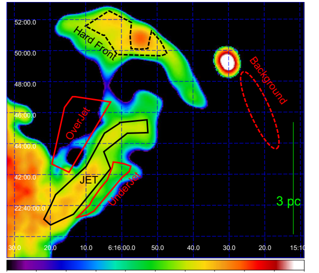
Fig. 2. Close-up view of the jet area marked by the cyan box in Fig. 1 in the Soft band (0.5–1.4 keV, top ) and in the Hard band (1.4–5 keV, bottom ). The image is adaptively smoothed to a signal-to-noise ratio 25, the bin size is 6'' and the color scale is logarithmic. Jet region is marked in black, Soft Front and Hard Front are marked in dashed black, background region in dashed red and OverJet and UnderJet regions in red.
