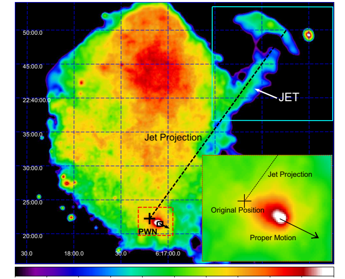
Fig. 1. Background-subtracted and vignetting-corrected count-rate images of IC 443 in the Hard band (1.4–5 keV) obtained by combining all the EPIC cameras. The image is adaptively smoothed to a signal-to-noise ratio of 25, the bin size is 6'' and the color scale is logarithmic. In the upper panel , the black box marks the PWN (and the field of view of Fig. 3), the black arrows marks the proper motion of the PWN, the black cross indicates the original position of the PWN (immediately after the explosion) and the white contours traces the molecular cloud as reported by Burton et al. (1988) . In the lower panel , the cyan box marks the jet (and the field of view of Fig. 2), the dashed black line is the projection of the jet toward the PWN and the dashed red box is the FOV of the PWN area with the original position and proper motion marked by the black cross and black arrow, respectively.
