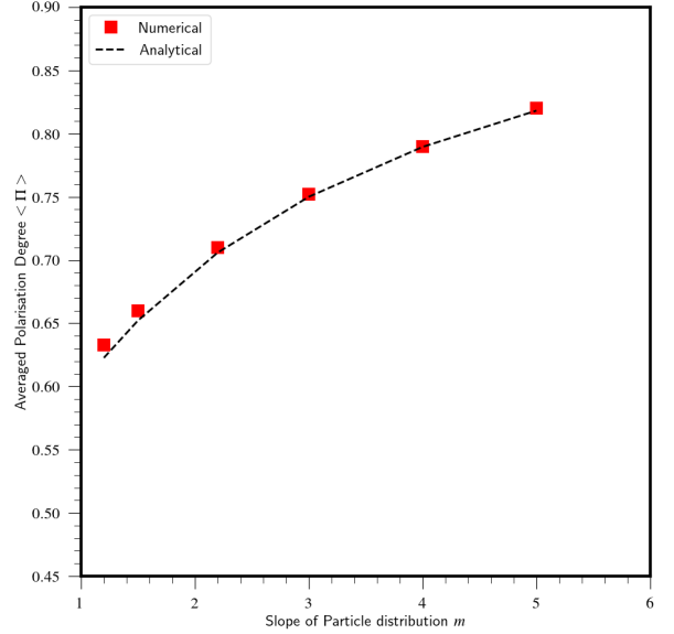
Figure 8. Comparison of the numerically estimated averaged ratio of J_{sy}(\nu) with J_{pol}(\nu) for \nu = 10^{10} GHz (red squares) with the theoretical values obtained from Eq.61 shown as black dashed line.
