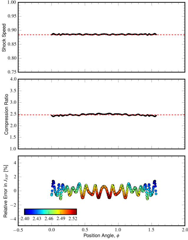
Figure 5. The variation of shock properties with angular position for the RMHD blast wave test. The shock velocity obtained from a single representative macro-particle is shown as black circles and the semi-analytical estimate from a very high resolution 1D run is shown as a red dash line in the top panel . The middle panel shows the variation of compression ratio obtained from the particles. The relative error in the estimate of mass flux, J_{\text{NIF}} in the normal incidence frame is shown in the bottom panel , the colors here indicate the value of compression ratio.
