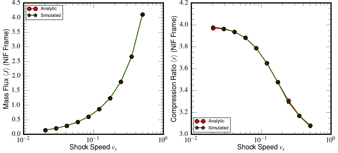
Figure 3. Left panel : Analytical mass flux J in the lab frame (or NIF) estimated from Eq. (19) is shown as (red dots), whereas its average value \langle J \rangle obtained from macro-particles are shown as green stars. In the right panel , the analytical (red dots) and simulated values of compression ratio, r (green stars) estimated using Eq. (B13) are shown. The simulated values are obtained as macro-particles traverse the relativistic planar shock and the sampled quantities across the shock are transformed to a shock rest frame (see text).
