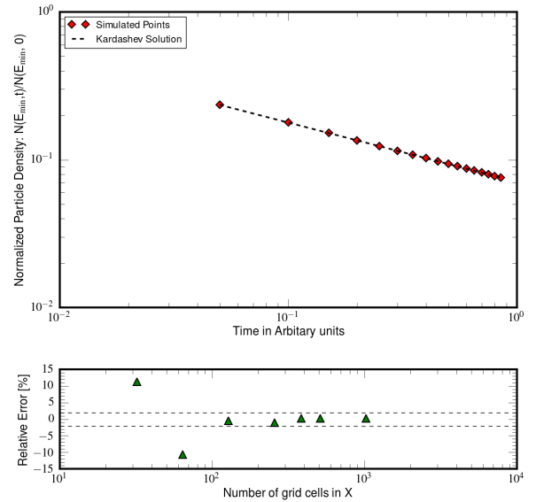
Figure 7. Top Comparing the temporal evolution of normalized spectral distribution, \mathcal{N}(E_{\min}, t) (red squares) with analytical solution obtained from Eq. 58 shown as black dashed line. Bottom Results from the convergence study with different resolution are shown in this panel. The green triangles represent the relative errors (%) in estimating the analytical slope for the variation of \mathcal{N}(E_{\min}, t) with respect to time. The two black dashed line marks the \pm 2\% error.
