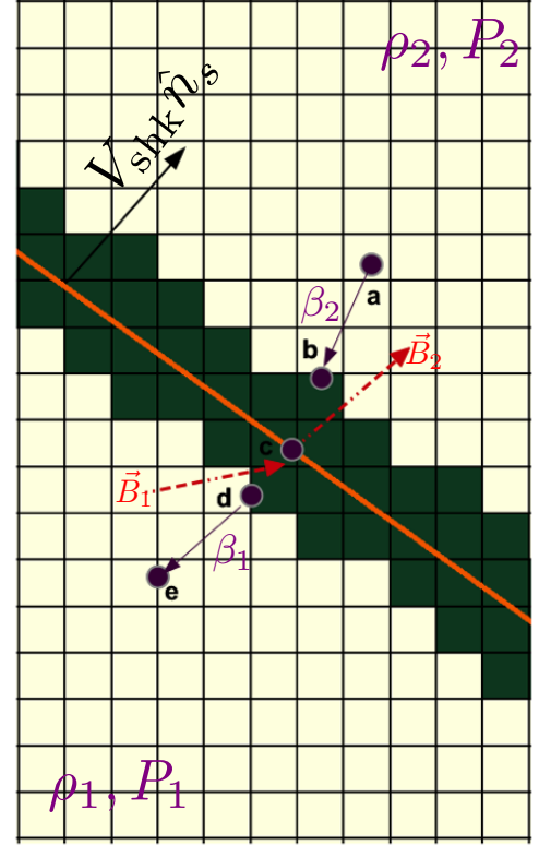
Figure 1. Cartoon figure showing the different positions of the particle and corresponding diagnostics
