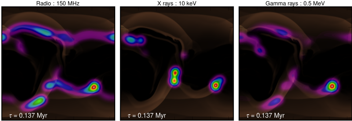
Figure 13. Multi-wavelength emission signatures from slab jet simulation run at time \tau = 0.137 \text{ Myr} . Every panel shows the fluid density \rho (as copper colors). The emissivities shown in each panel are obtained from instantaneous spectral distribution of particles and deposited on the grid. They are shown in spectral colors for three different observed frequencies viz., \nu = 150 \text{ MHz} (left), 10 \text{ keV} (middle) due to synchrotron processes and 0.5 \text{ MeV} (right) due to Inverse Compton.
