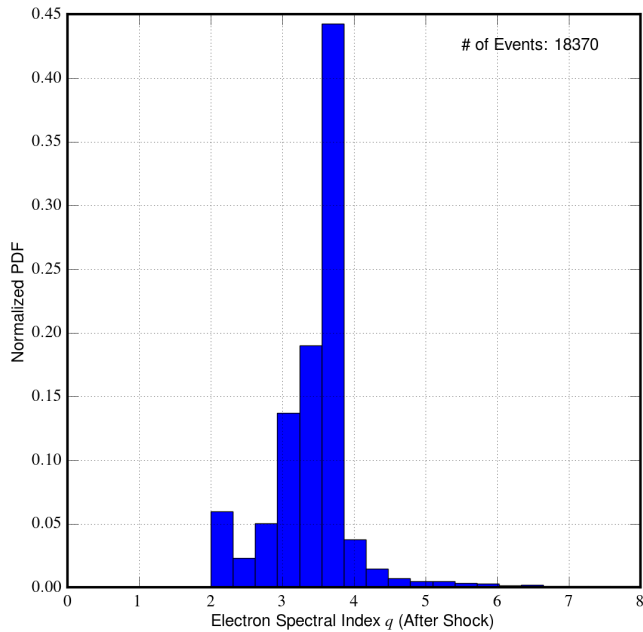
Figure 12. Normalized PDF of the modified spectral slope q as the particle crosses the shock during the evolution of slab jet until 0.3 Myr.
