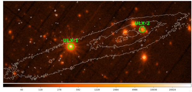
Figure 1. XMM-Newton stacked image of NGC 55. Circles with 20 arcsec radii are drawn around the ULXs along with surface brightness contours from the filter-RG610 DSS 2 image. The colour bar shows the number of counts.
