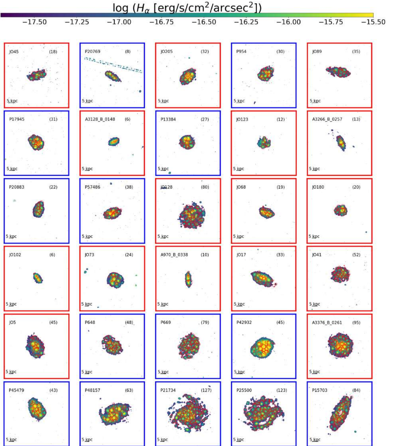
Figure 7. H\alpha maps for all galaxies in the sample, sorted by increasing stellar mass. Red circles show the H\alpha knots. Galaxies surrounded by a red square belong to clusters, and galaxies surrounded by a blue square belong to the field. Numbers in parenthesis are the number of knots in each galaxy.
