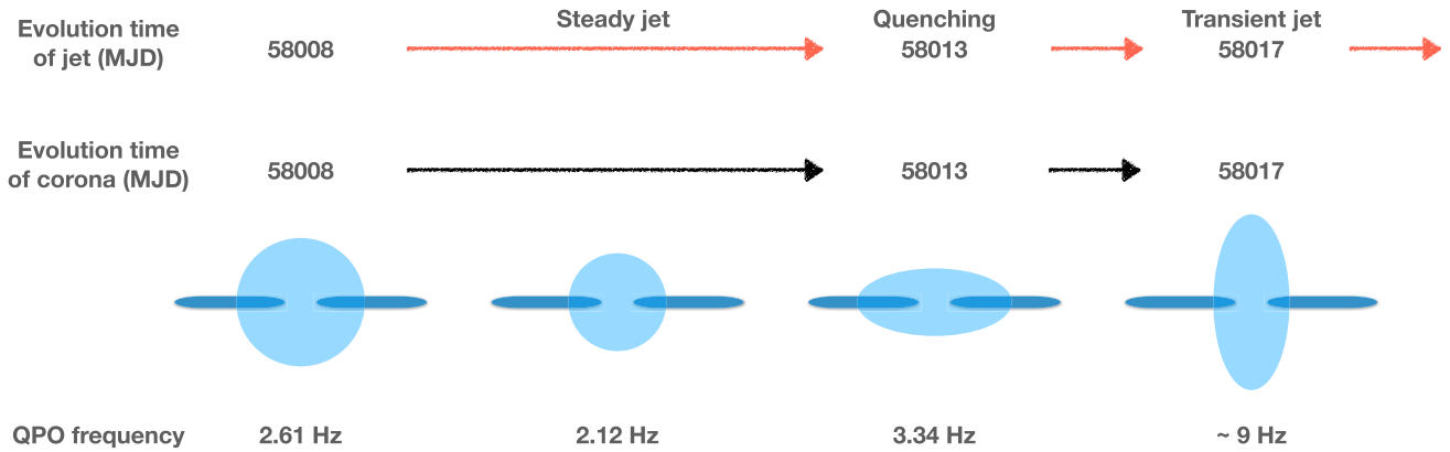
Figure 6. Schematic figure illustrating the time evolution of the corona and the jet of MAXI J1535–571 (see text for a more detailed explanation). From MJD 58008 to MJD 58011 the size of the corona contracts; from MJD 58011 to MJD 58013 the corona contracts vertically but expands horizontally. In the period before MJD 58013, the radio spectrum of the source is consistent with optically thick synchrotron emission from a compact steady jet and on MJD 58013 the jet is quenched. From MJD 58013 to MJD 58017 the corona expands vertically but contracts horizontally and after MJD 58017 the radio data are consistent with optically thin synchrotron emission from a transient jet.
