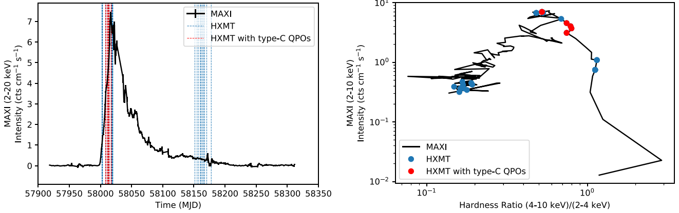
Figure 1. Left-hand panel: MAXI light curve of MAXI J1535–571 in black with the time of all the Insight -HXMT observations indicated by the vertical dashed lines. The selected MJD range of MAXI observations is from 57918 to 58312. The red dashed lines represent the observations that we analyse with type-C QPOs in the intermediate state. Right-hand panel: Hardness intensity diagram (HID) of MAXI J1535–571 using MAXI data in black. The selected MJD range of MAXI observations is from 57997 to 58174. The blue and red points indicate the simultaneous Insight -HXMT observations. The red points represent the observations that we analyse with type-C QPOs in the intermediate state. Note that some of the red points overlap each other. There are three red points in the left group and five red points in the right group.
