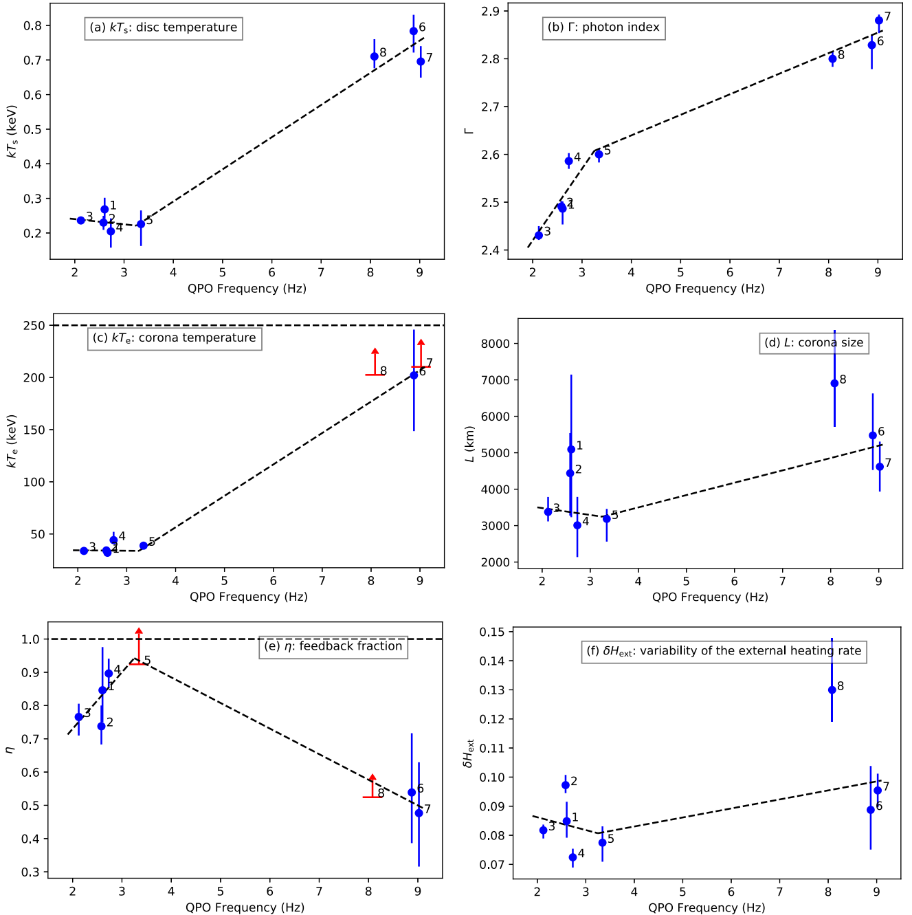
Figure 4. The evolution of the parameters of MAXI J1535–571 versus QPO frequency. The parameters are, respectively, (a) disc temperature, kT_s , (b) photon index, \Gamma , (c) corona temperature, kT_e , (d) corona size, L , (e) feedback fraction, \eta , and (f) variability of the external heating rate, \delta\dot{H}_{\text{ext}} . The error bars represent the 90 per cent confidence level, while red points show 95 per cent lower limits. Black dashed broken line is the best fit to the data by a broken line with a break frequency at 3.25 Hz. The numbers on each panel indicate the observations in Table 1. The horizontal black dashed lines in panels (c) and (e) are the upper boundaries of 250 keV and 1, respectively.
