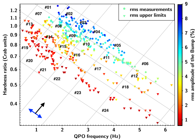
Figure 2. Hardness ratio versus QPO frequency for the 410 observations of GRS 1915+105. The coloured points indicate the rms amplitude of the bump. The black and blue arrows indicate the directions in which the rms amplitude of the bump increases and remains broadly constant, respectively. The plot is divided into different regions of regular intervals on the hardness ratio and QPO frequency (see Table A1 for details on the division and the observations in each group).
